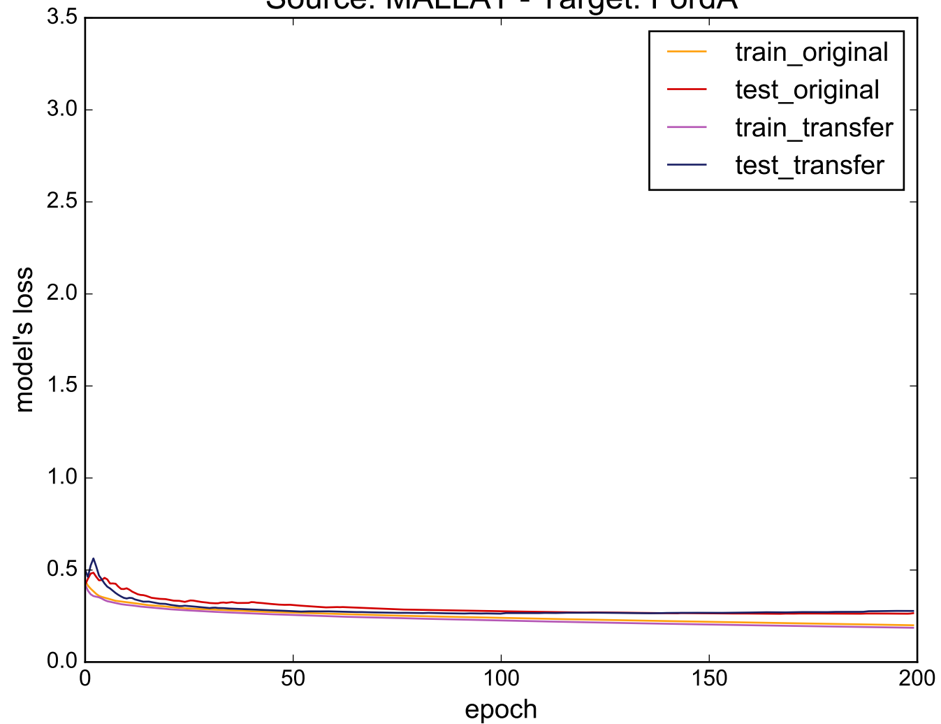
Source: MALLAT - Target: FordA
