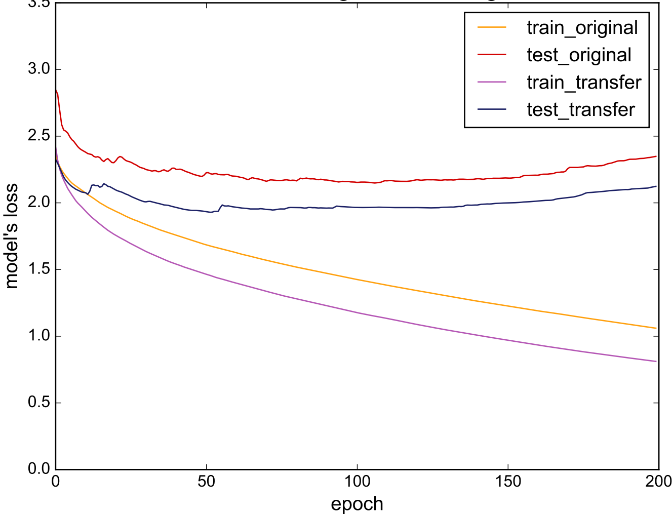
Source: MALLAT - Target: InsectWingbeatSound
