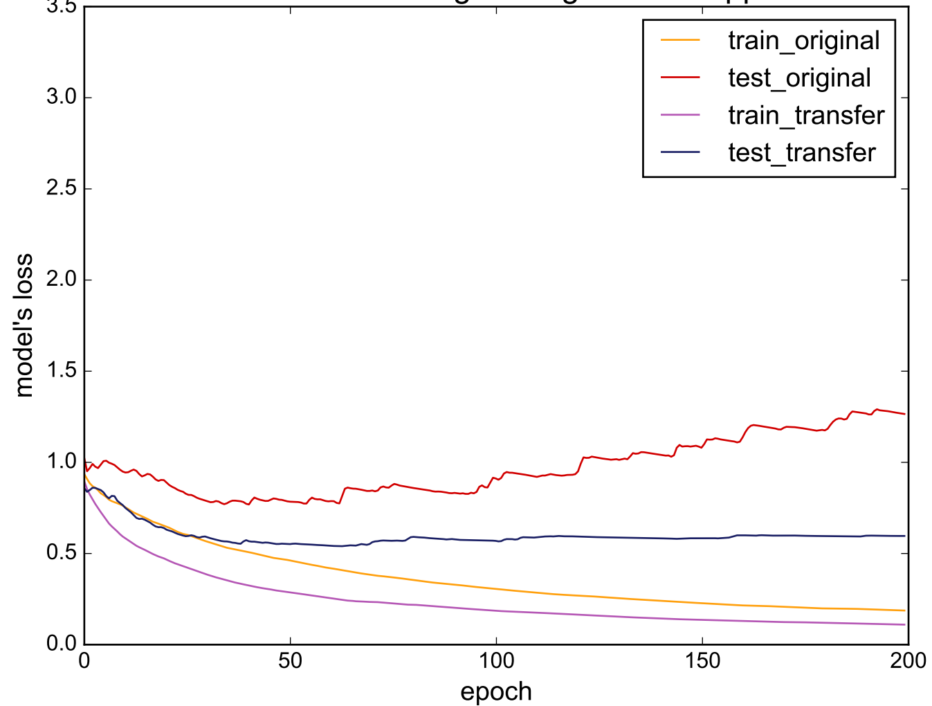
Source: MALLAT - Target: LargeKitchenAppliances
