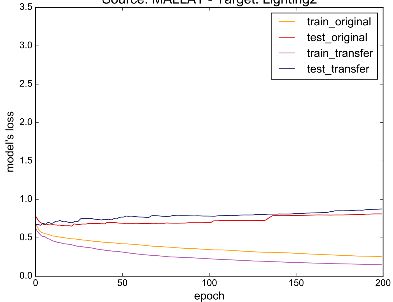
Source: MALLAT - Target: Lighting2
