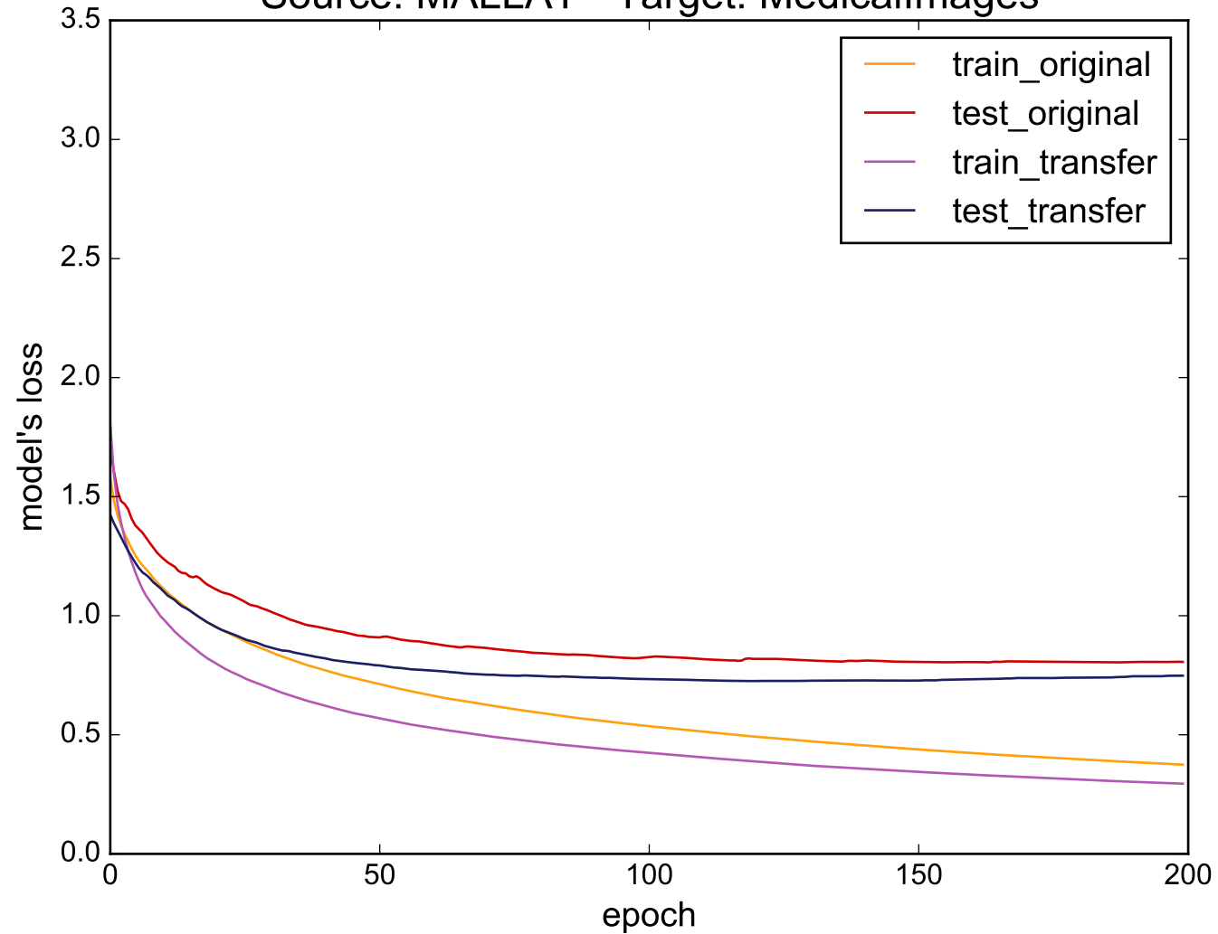
Source: MALLAT - Target: MedicalImages
