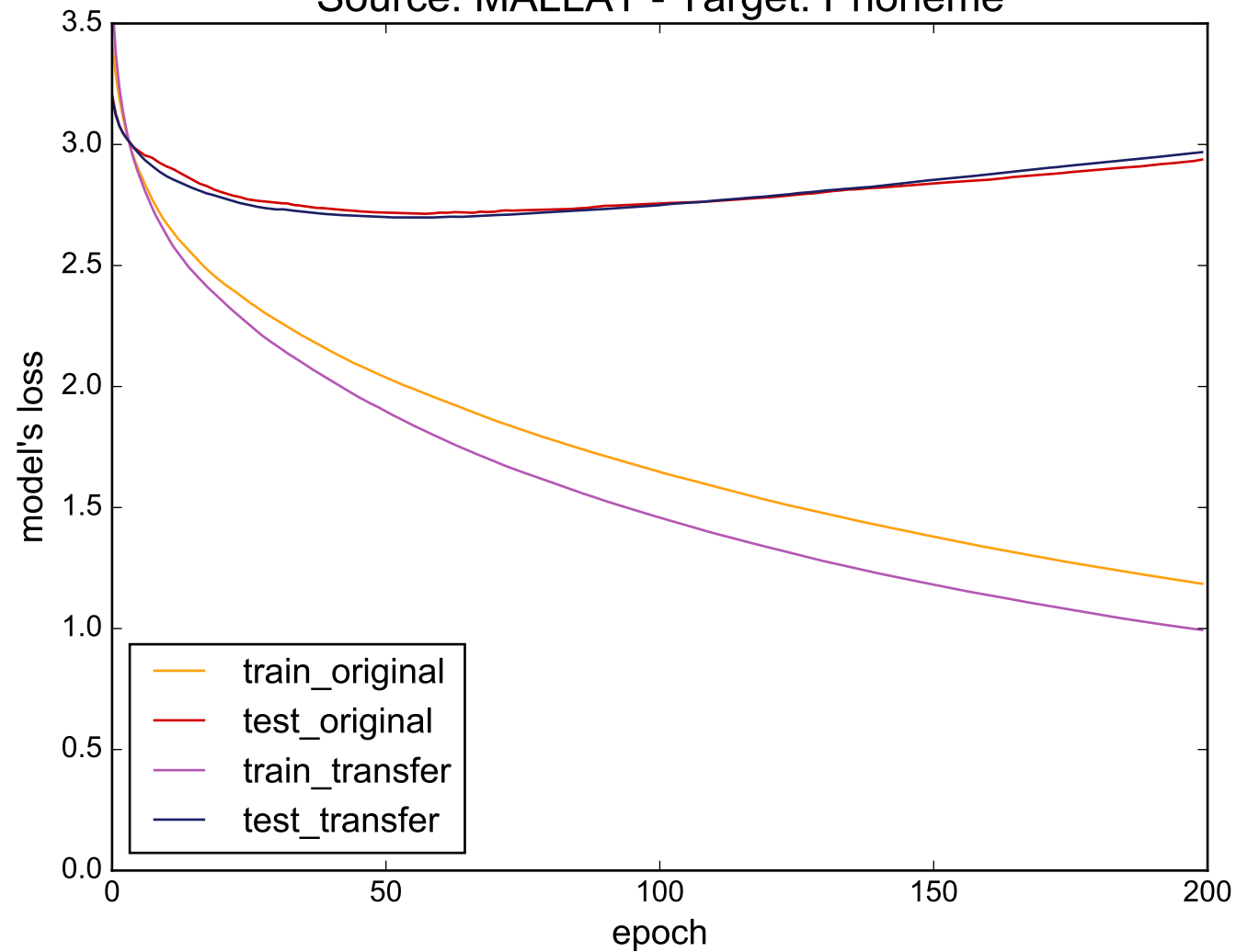
Source: MALLAT - Target: Phoneme
