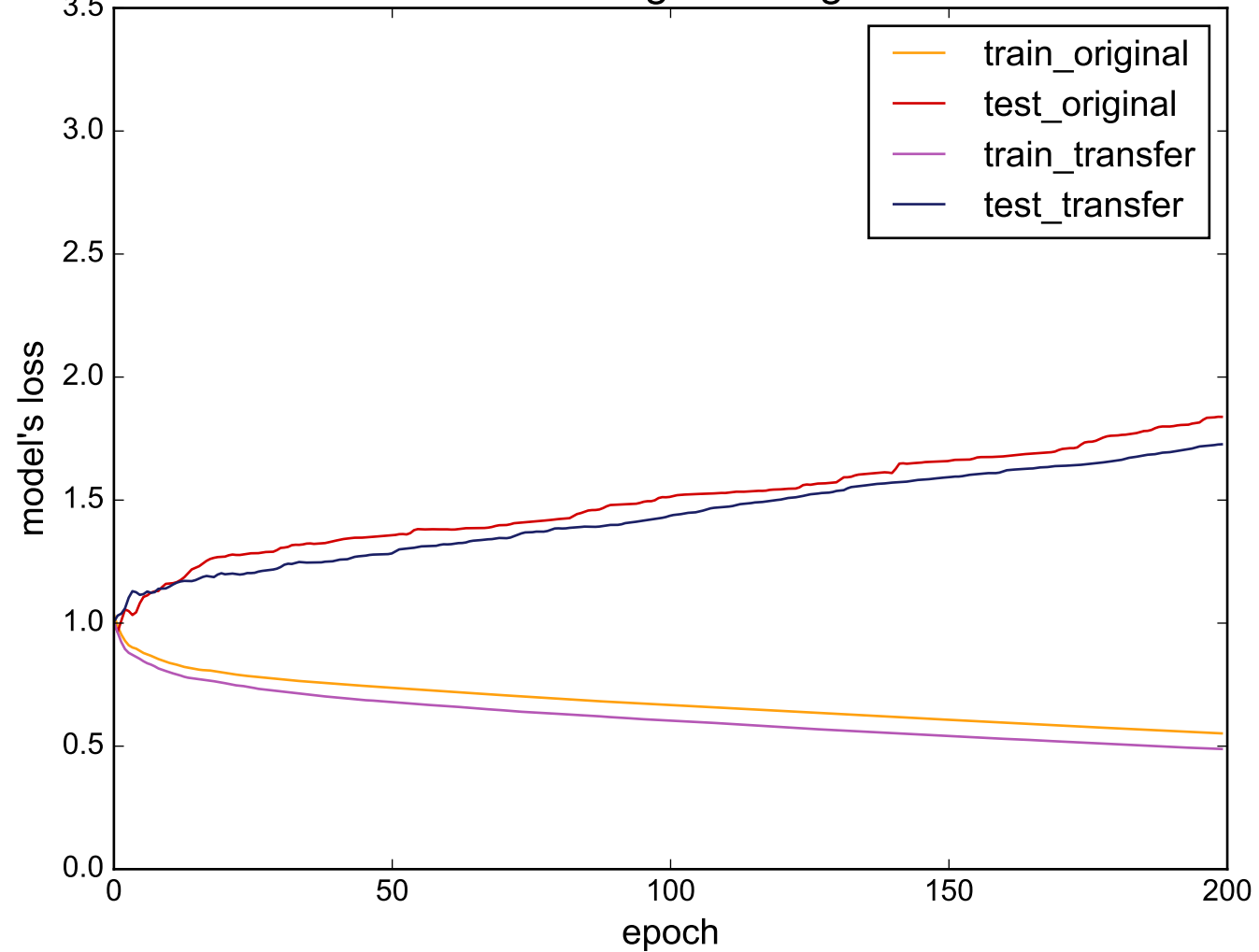
Source: MALLAT - Target: RefrigerationDevices
