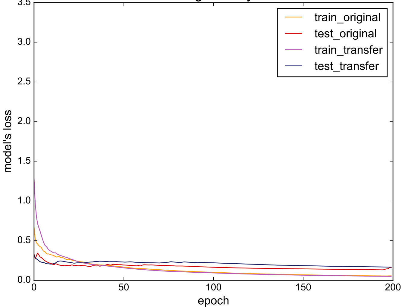
Source: MALLAT - Target: SonyAIBORobotSurface
