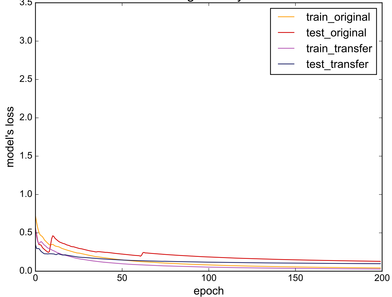
Source: MALLAT - Target: SonyAIBORobotSurfaceII
