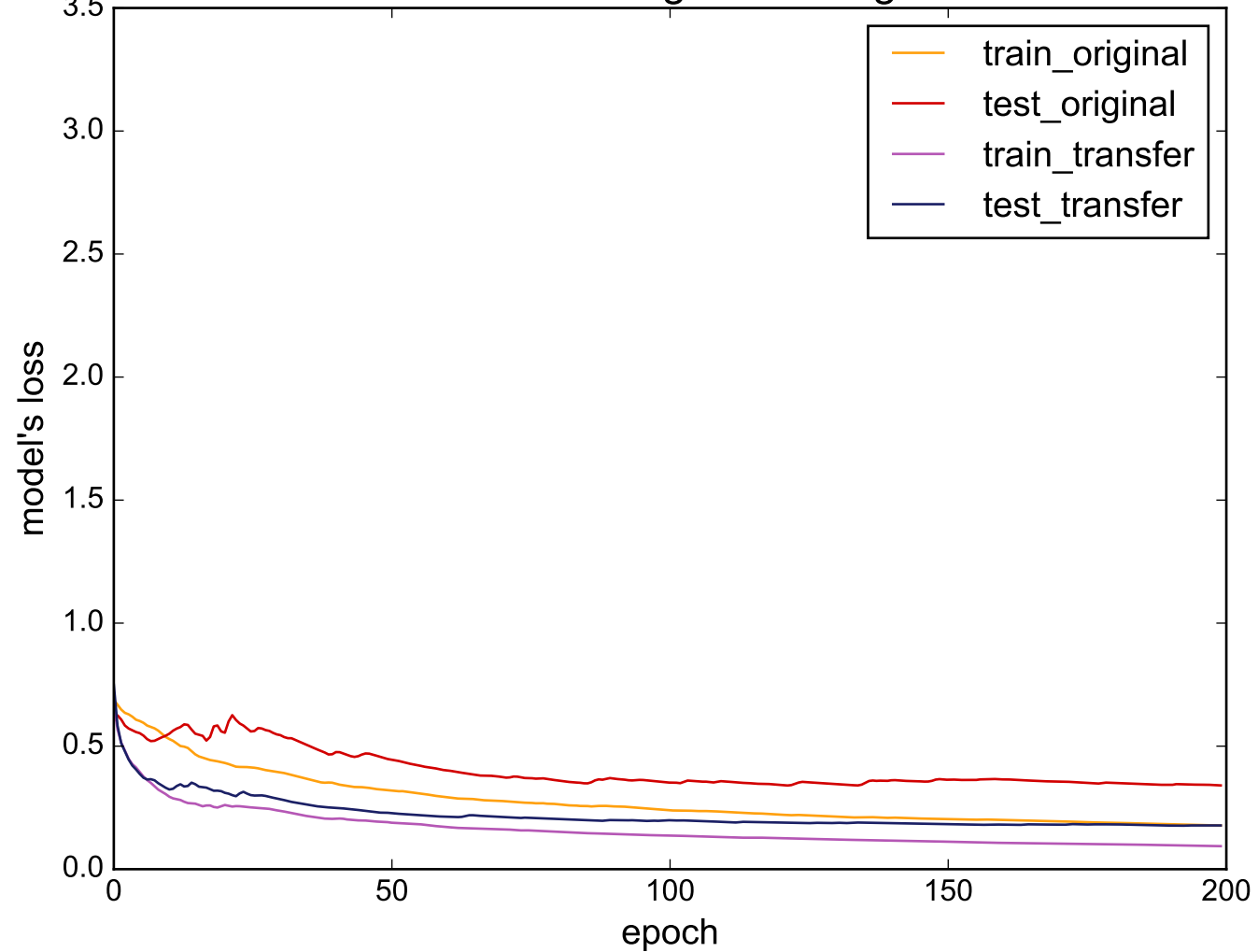
Source: MALLAT - Target: ToeSegmentation1
