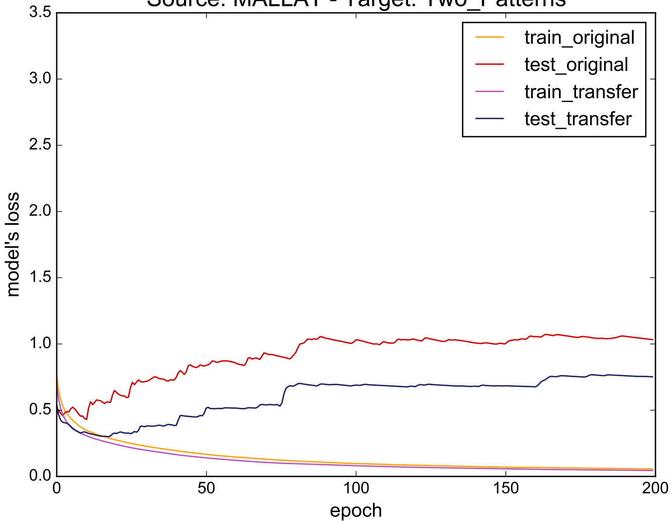
Source: MALLAT - Target: Two_Patterns
