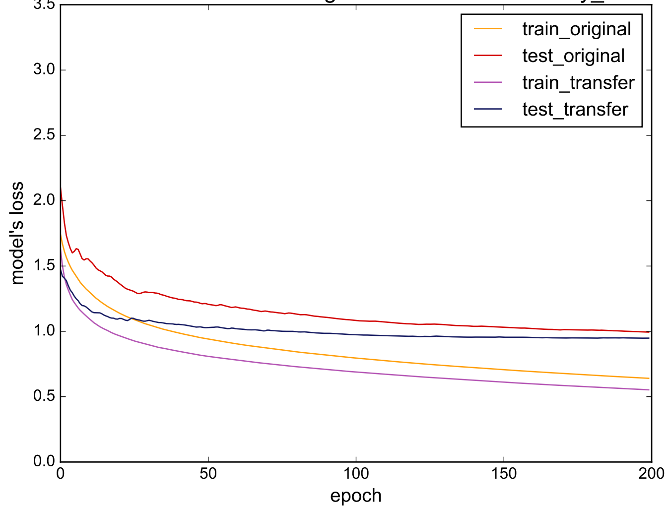
Source: MALLAT - Target: uWaveGestureLibrary_Z
