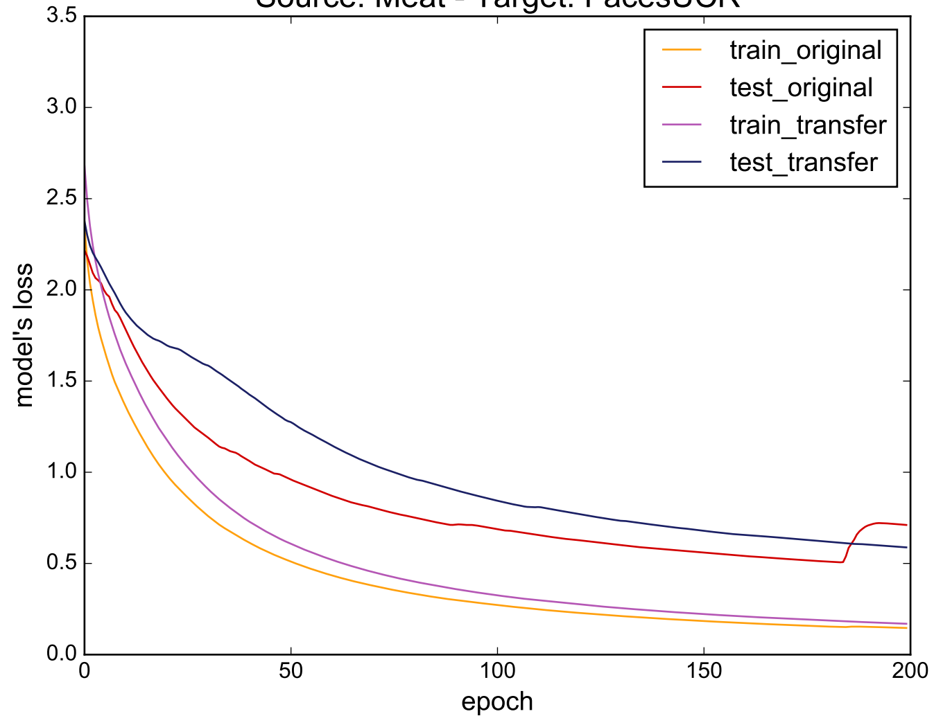
Source: Meat - Target: FacesUCR
