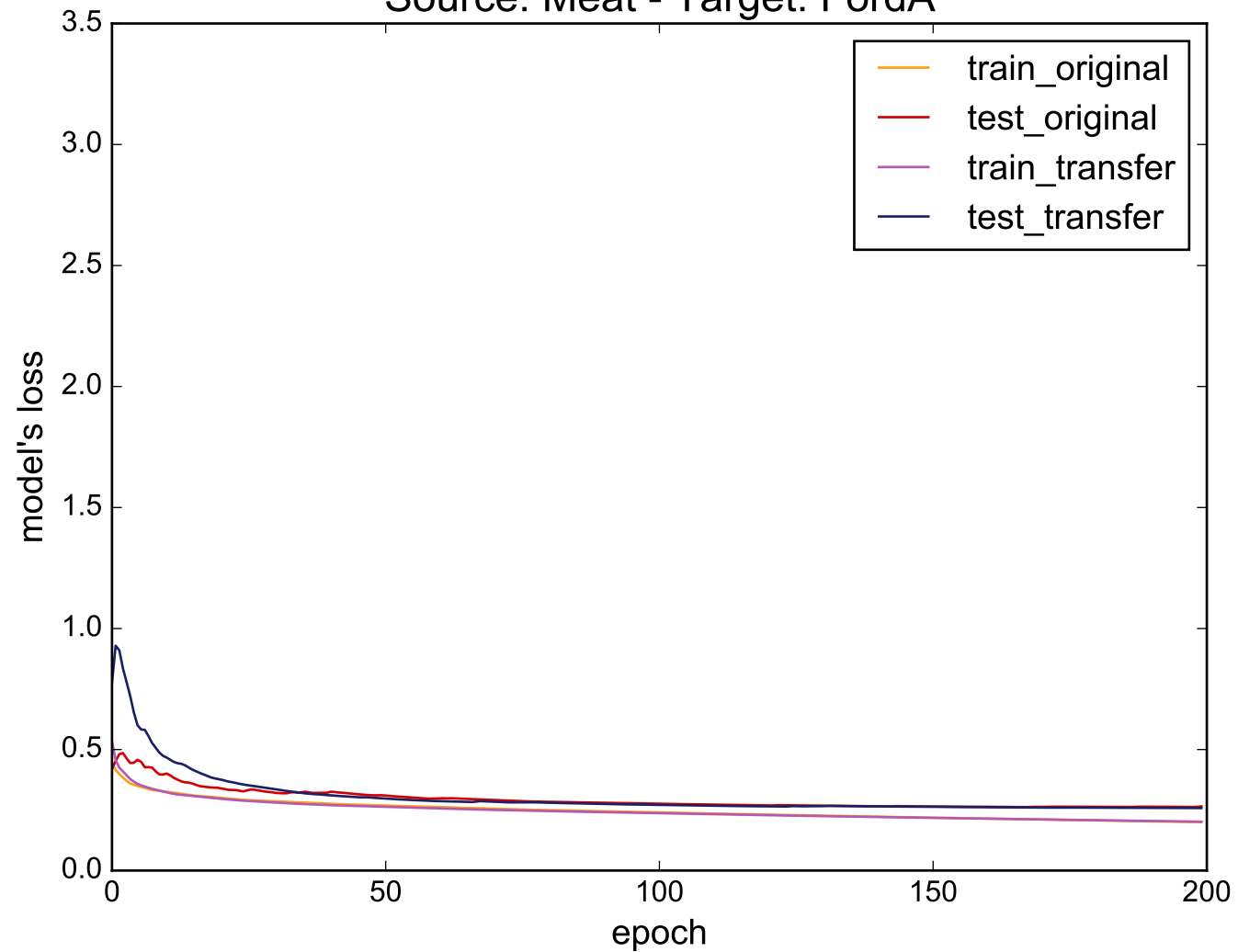
Source: Meat - Target: FordA
