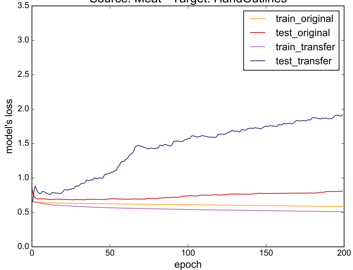
Source: Meat - Target: HandOutlines
