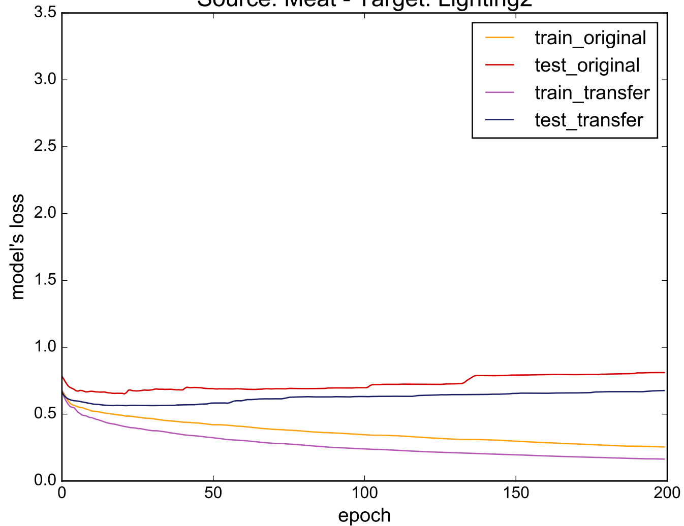
Source: Meat - Target: Lighting2
