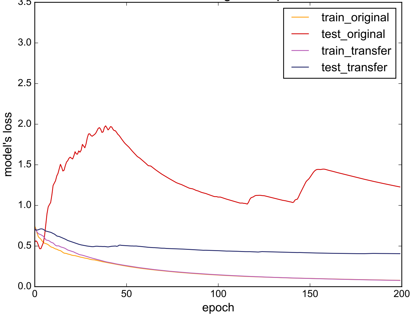
Source: Meat - Target: ShapeletSim
