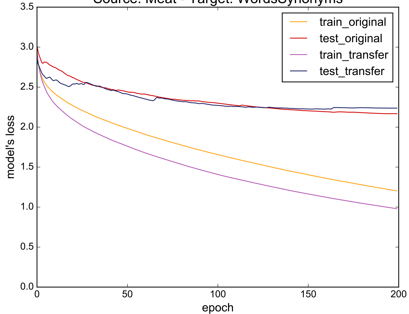
Source: Meat - Target: WordsSynonyms
