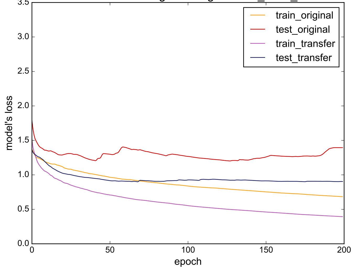
Source: MedicalImages - Target: CinC_ECG_torso
