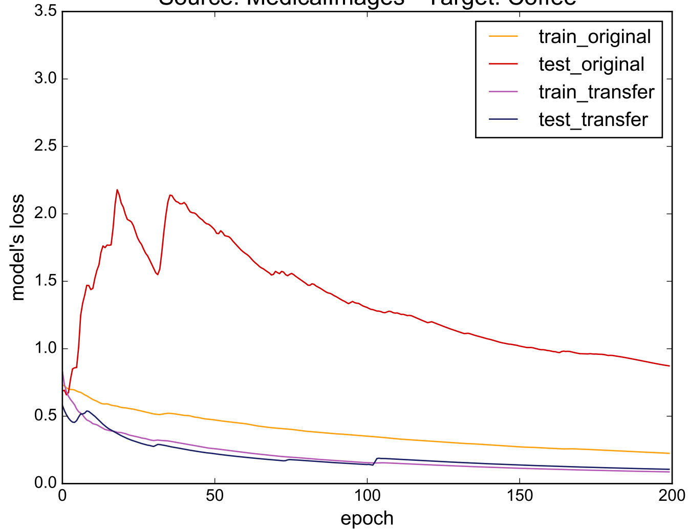
Source: MedicalImages - Target: Coffee
