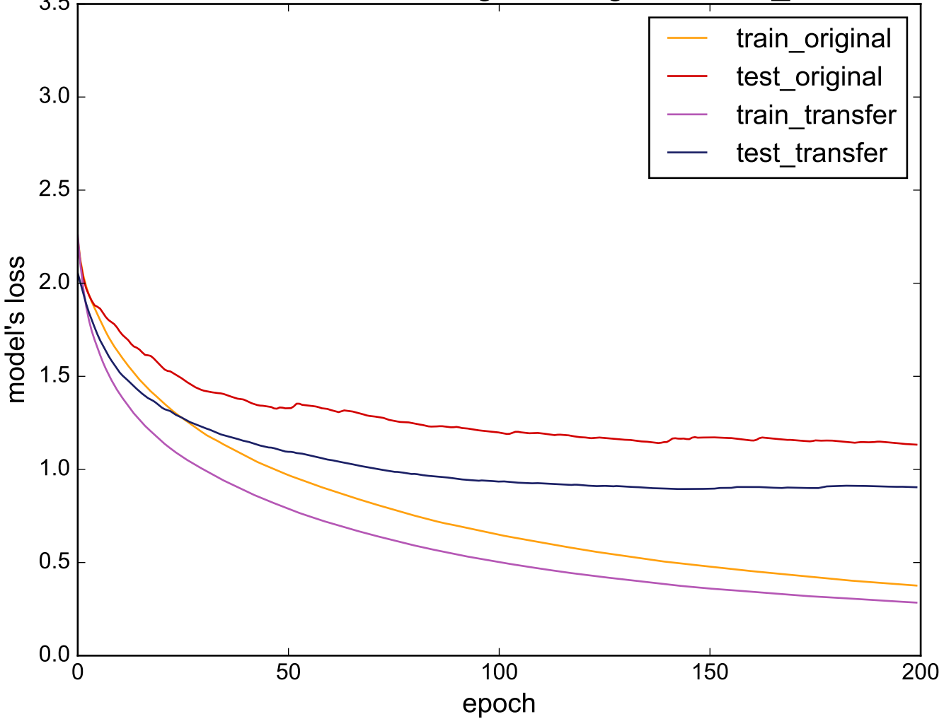
Source: MedicalImages - Target: Cricket_Y
