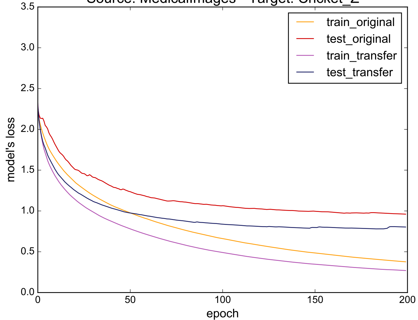
Source: MedicalImages - Target: Cricket_Z
