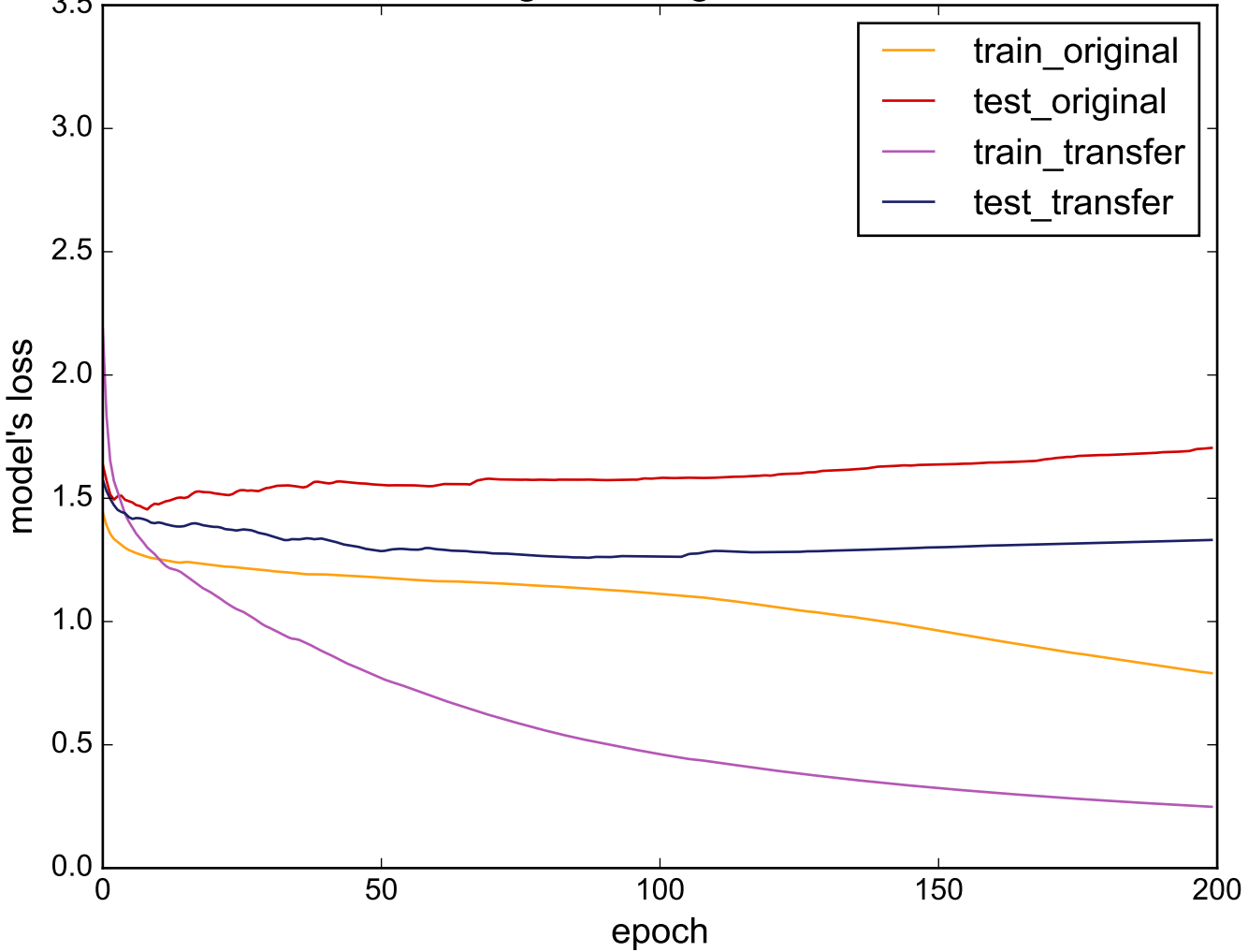
Source: MedicalImages - Target: DiatomSizeReduction
