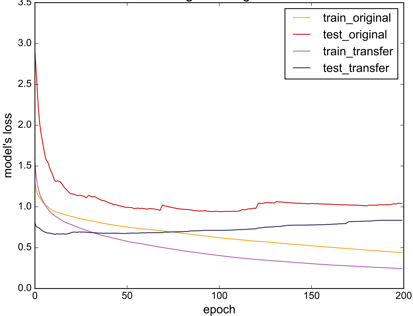
Source: MedicalImages - Target: DistalPhalanxTW
