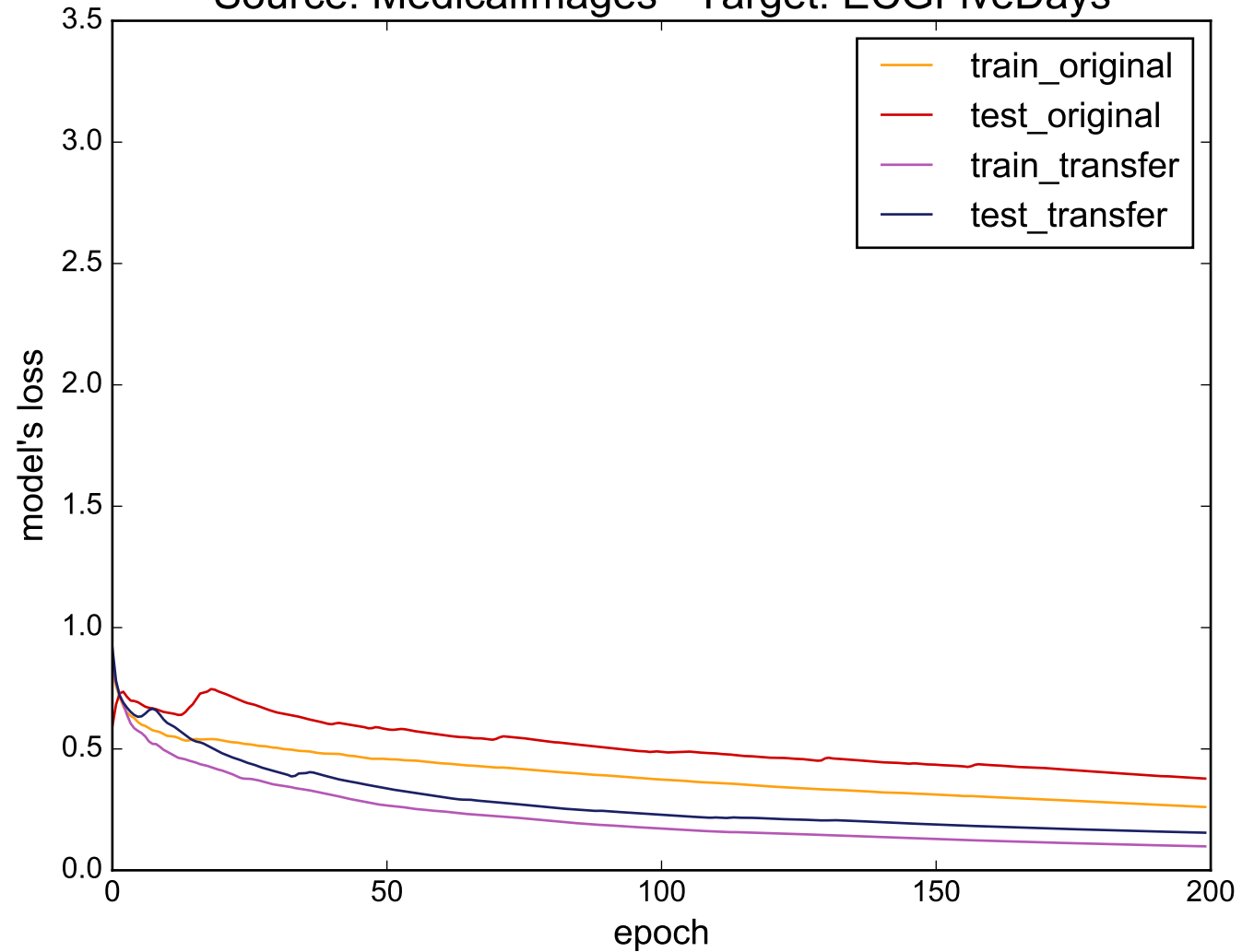
Source: MedicalImages - Target: ECGFiveDays
