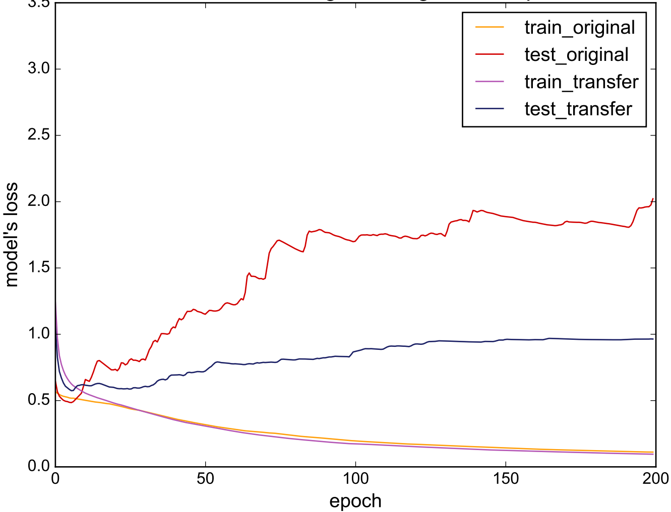
Source: MedicalImages - Target: Earthquakes
