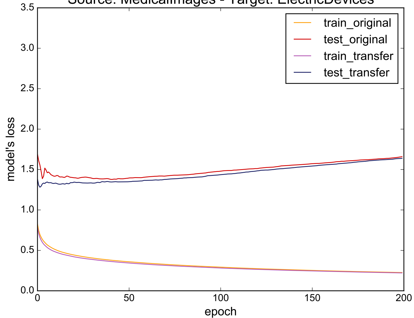
Source: MedicalImages - Target: ElectricDevices
