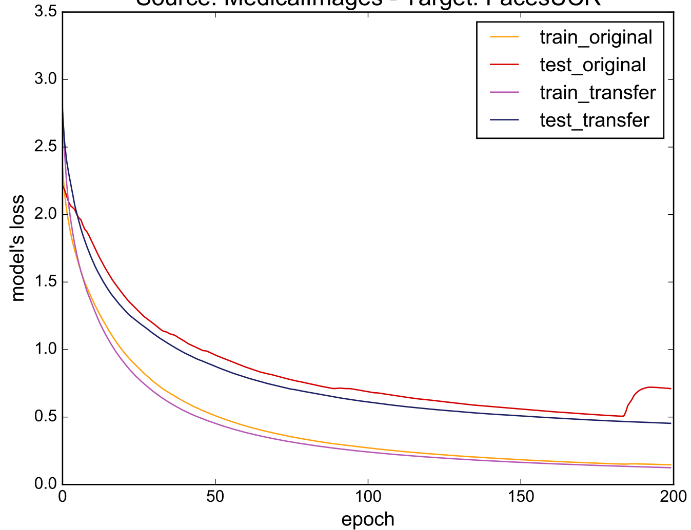
Source: MedicalImages - Target: FacesUCR
