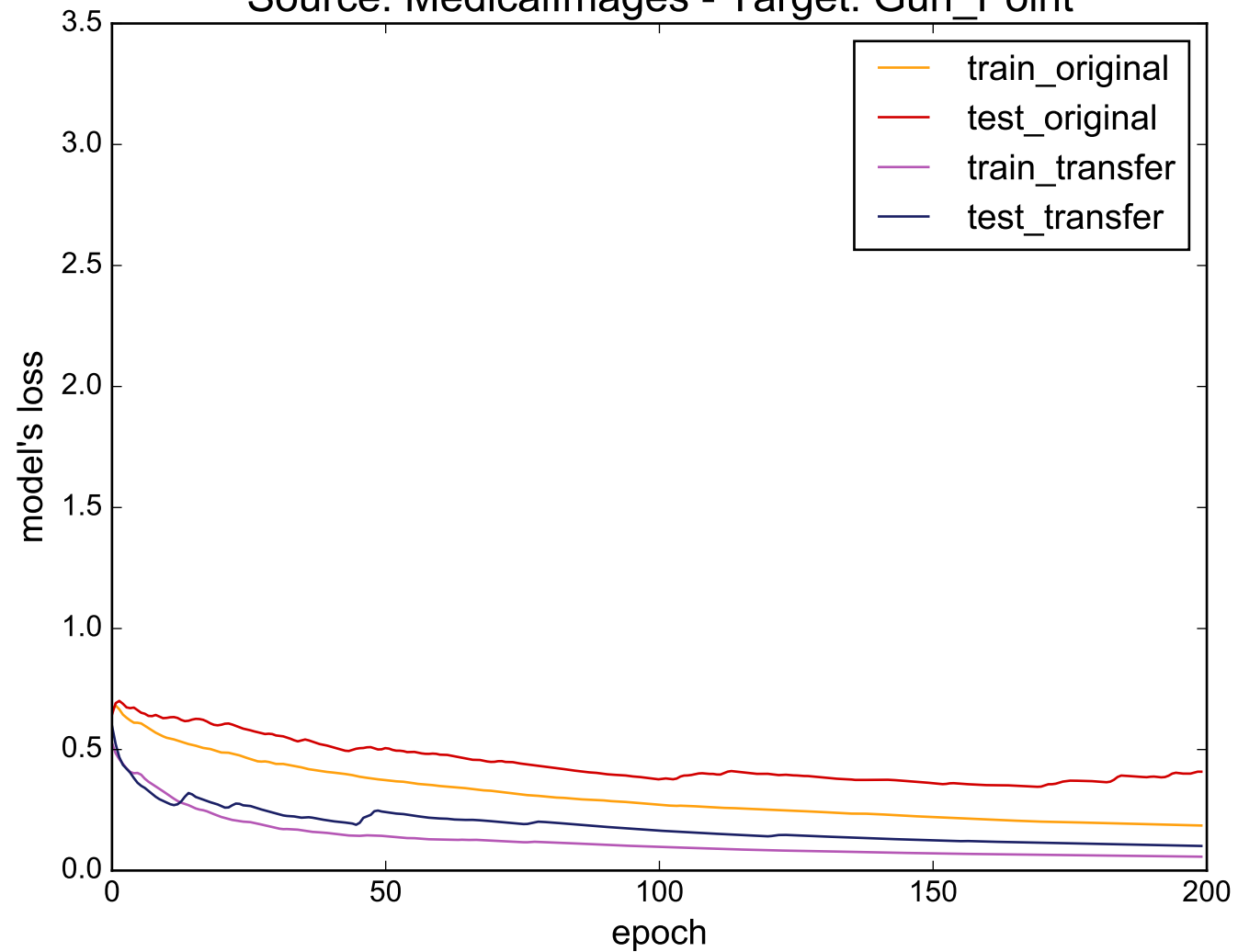
Source: MedicalImages - Target: Gun_Point
