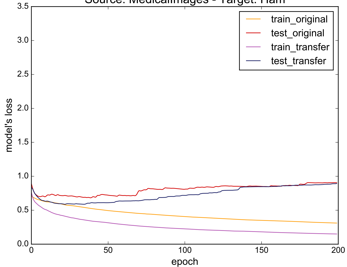
Source: MedicalImages - Target: Ham
