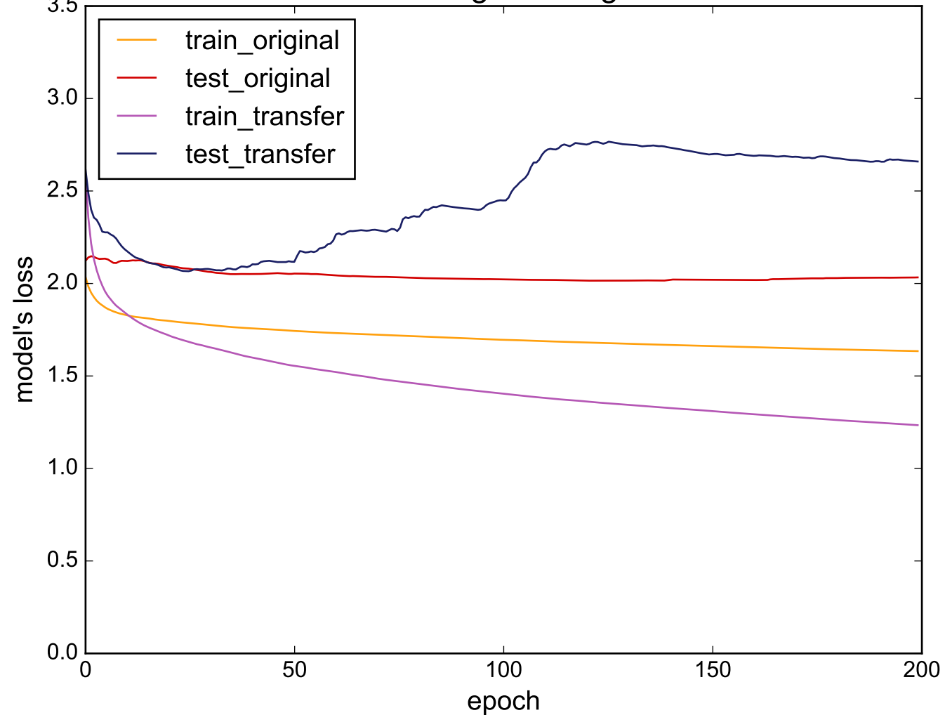
Source: MedicalImages - Target: InlineSkate
