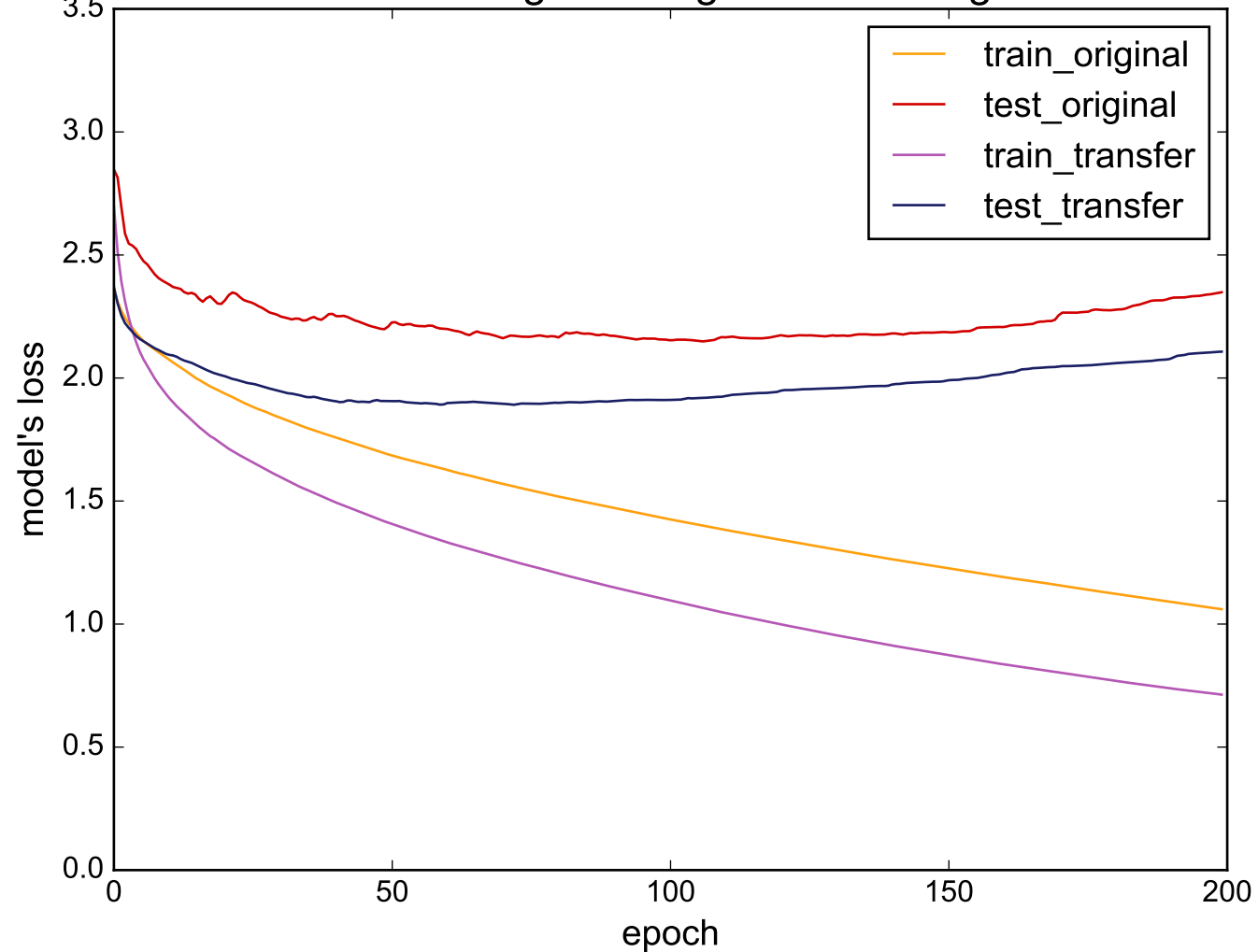
Source: MedicalImages - Target: InsectWingbeatSound
