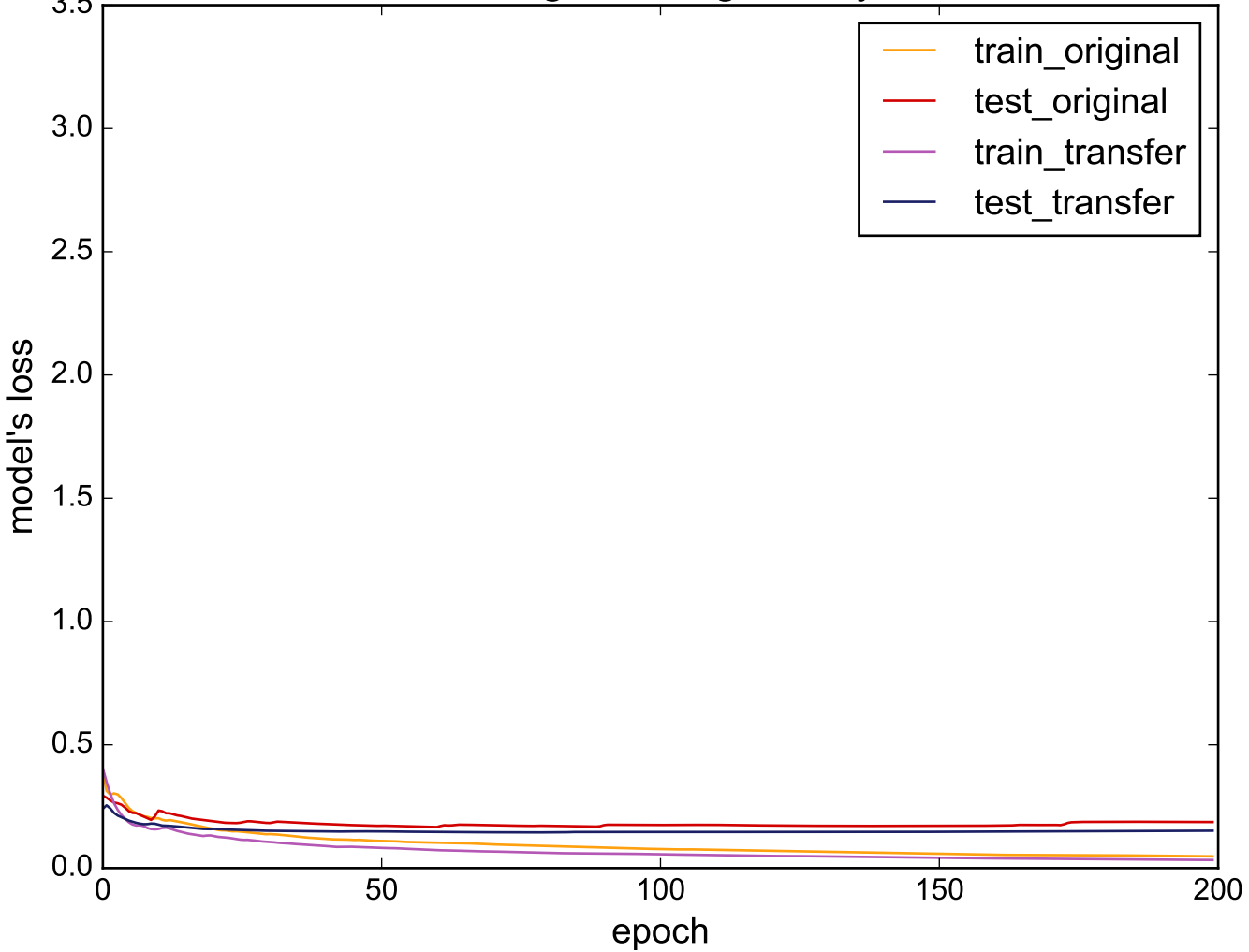
Source: MedicalImages - Target: ItalyPowerDemand
