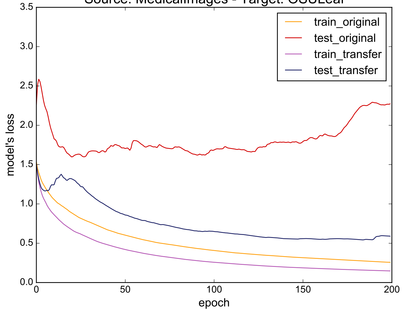
Source: MedicalImages - Target: OSULeaf
