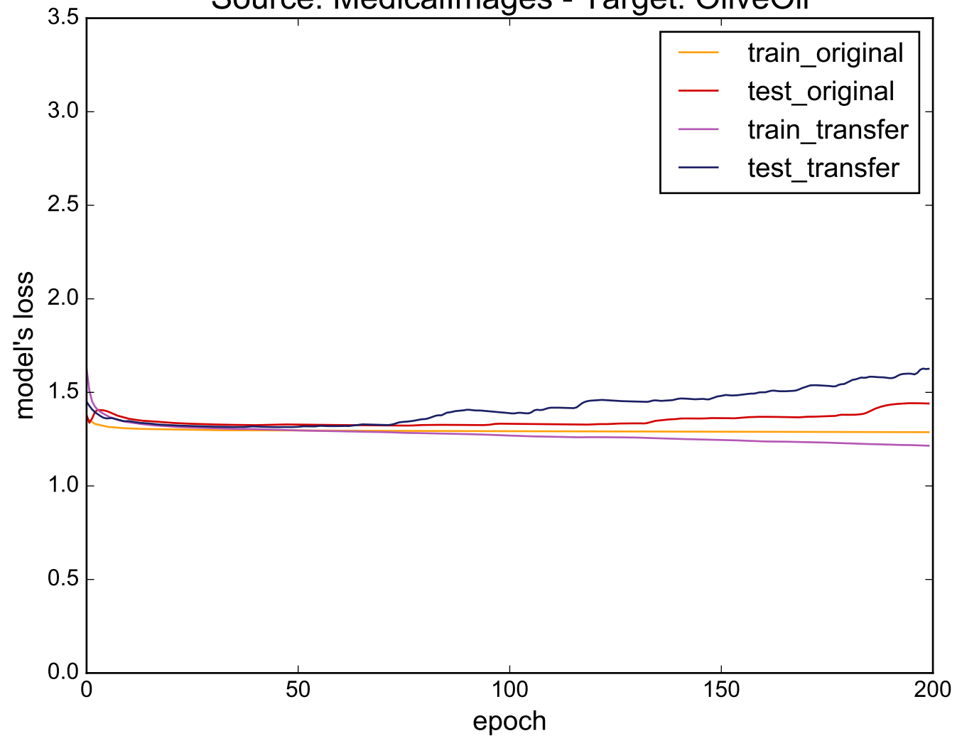
Source: MedicalImages - Target: OliveOil
