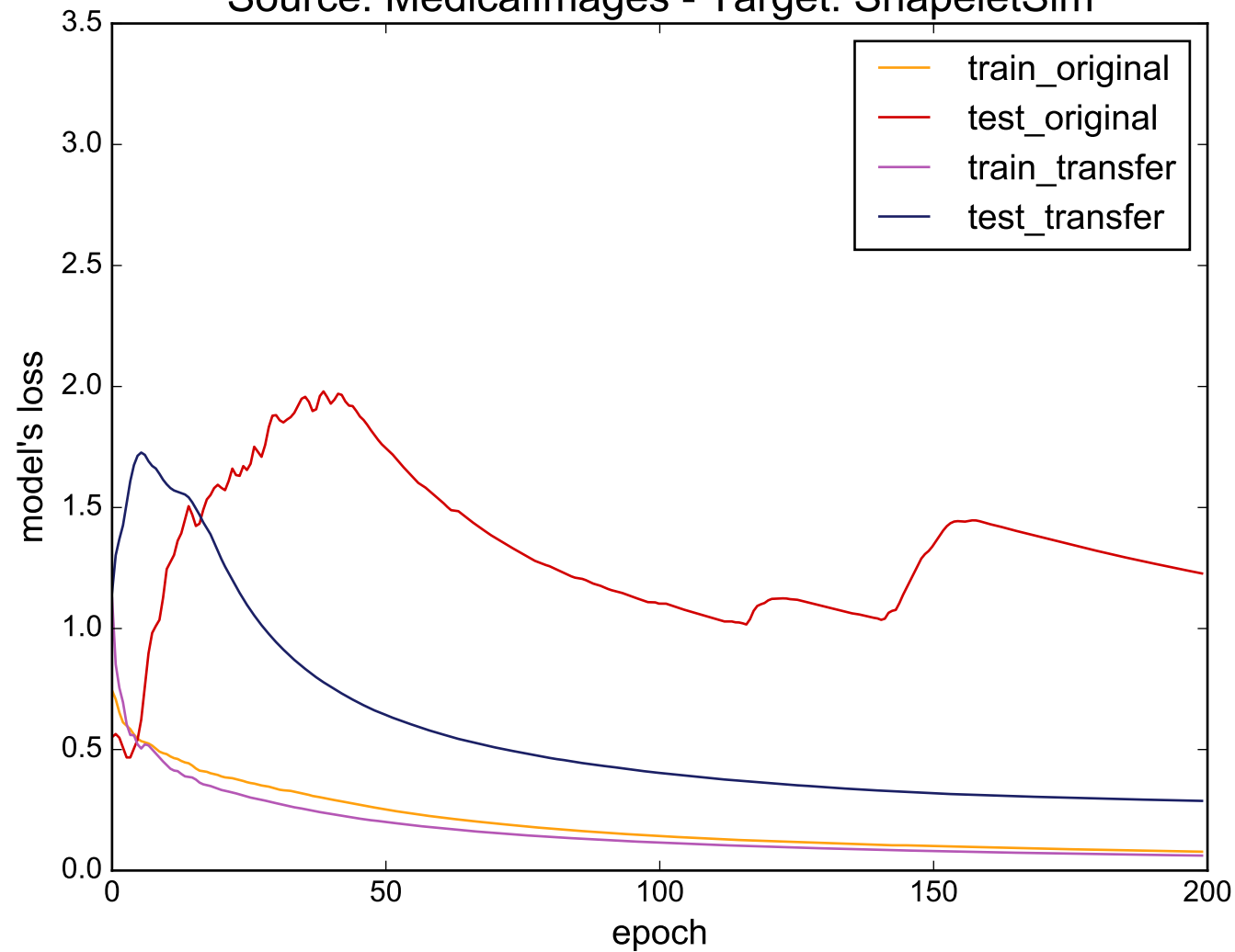
Source: MedicalImages - Target: ShapeletSim
