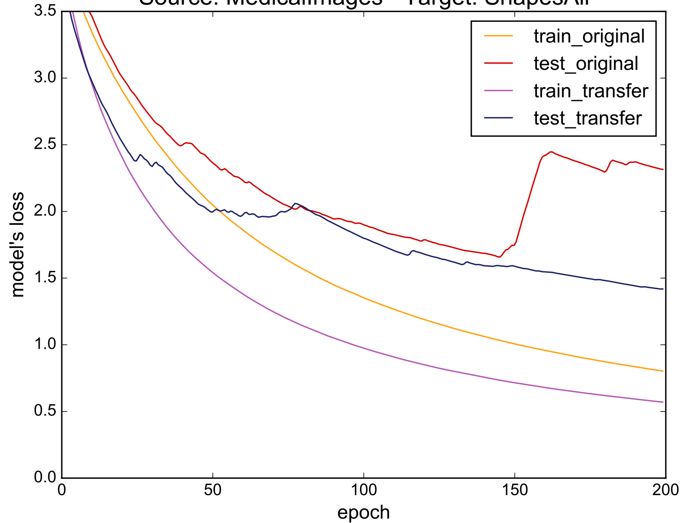
Source: MedicalImages - Target: ShapesAll
