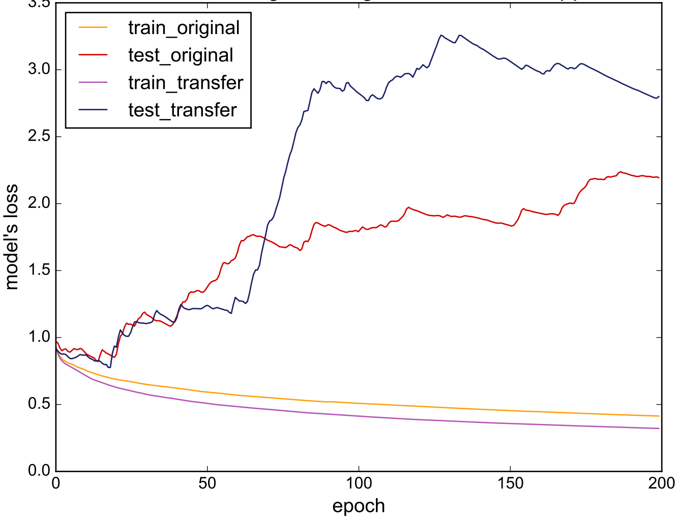
Source: MedicalImages - Target: SmallKitchenAppliances
