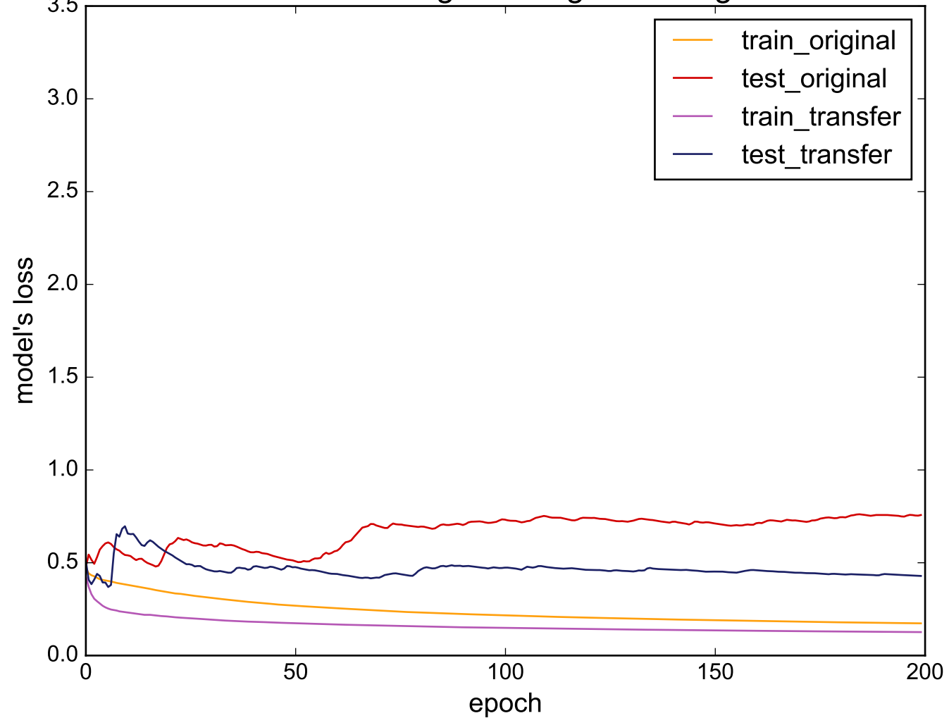
Source: MedicalImages - Target: StarLightCurves
