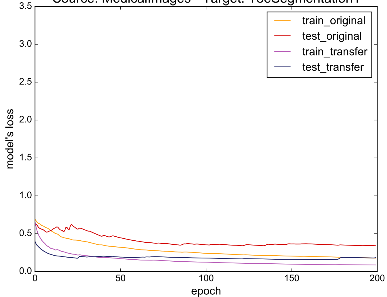
Source: MedicalImages - Target: ToeSegmentation1
