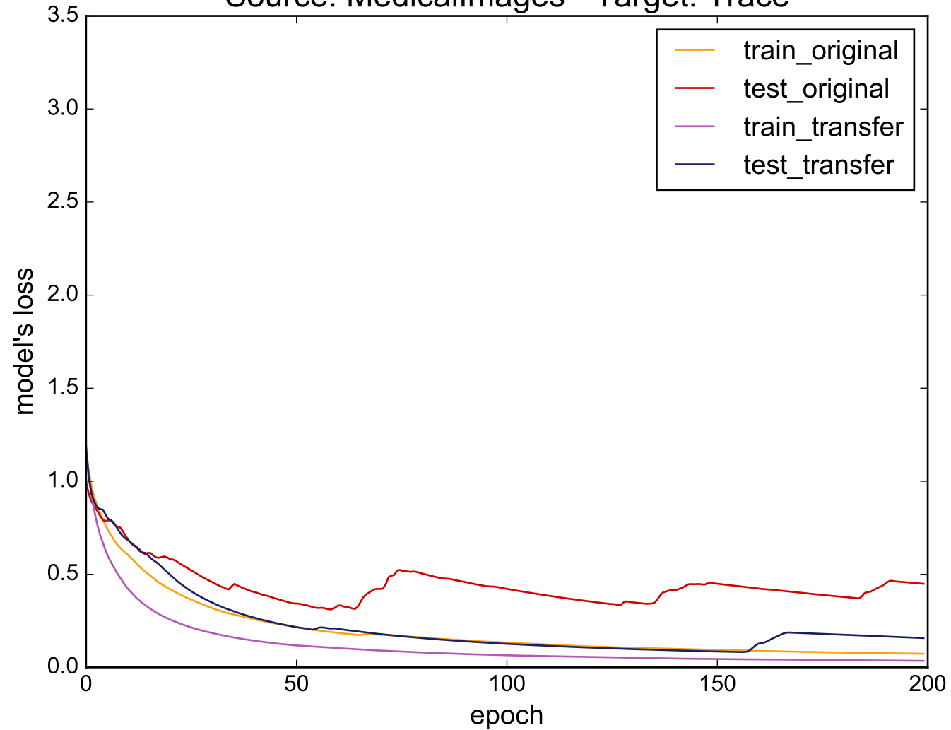
Source: MedicalImages - Target: Trace
