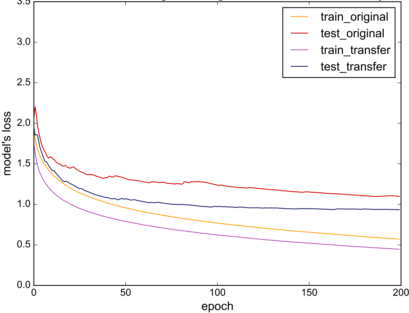
Source: MedicalImages - Target: UWaveGestureLibraryAll
