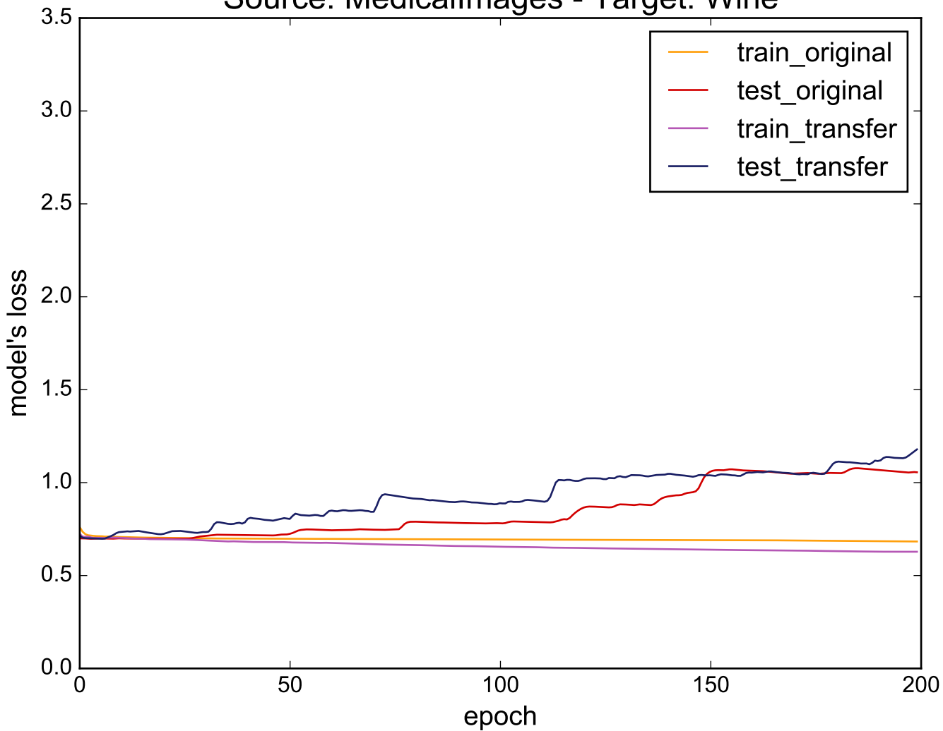
Source: MedicalImages - Target: Wine
