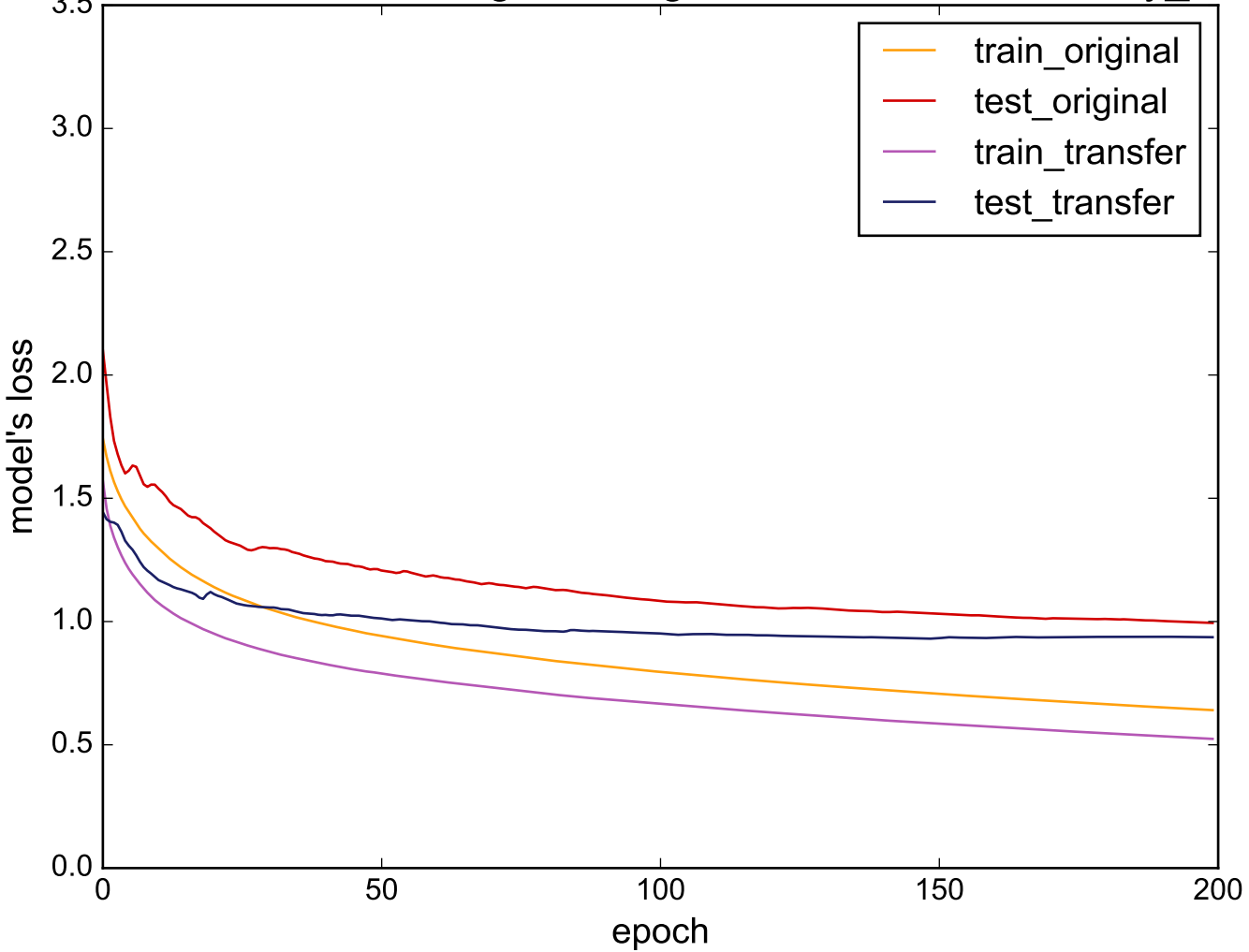
Source: MedicalImages - Target: uWaveGestureLibrary_Z
