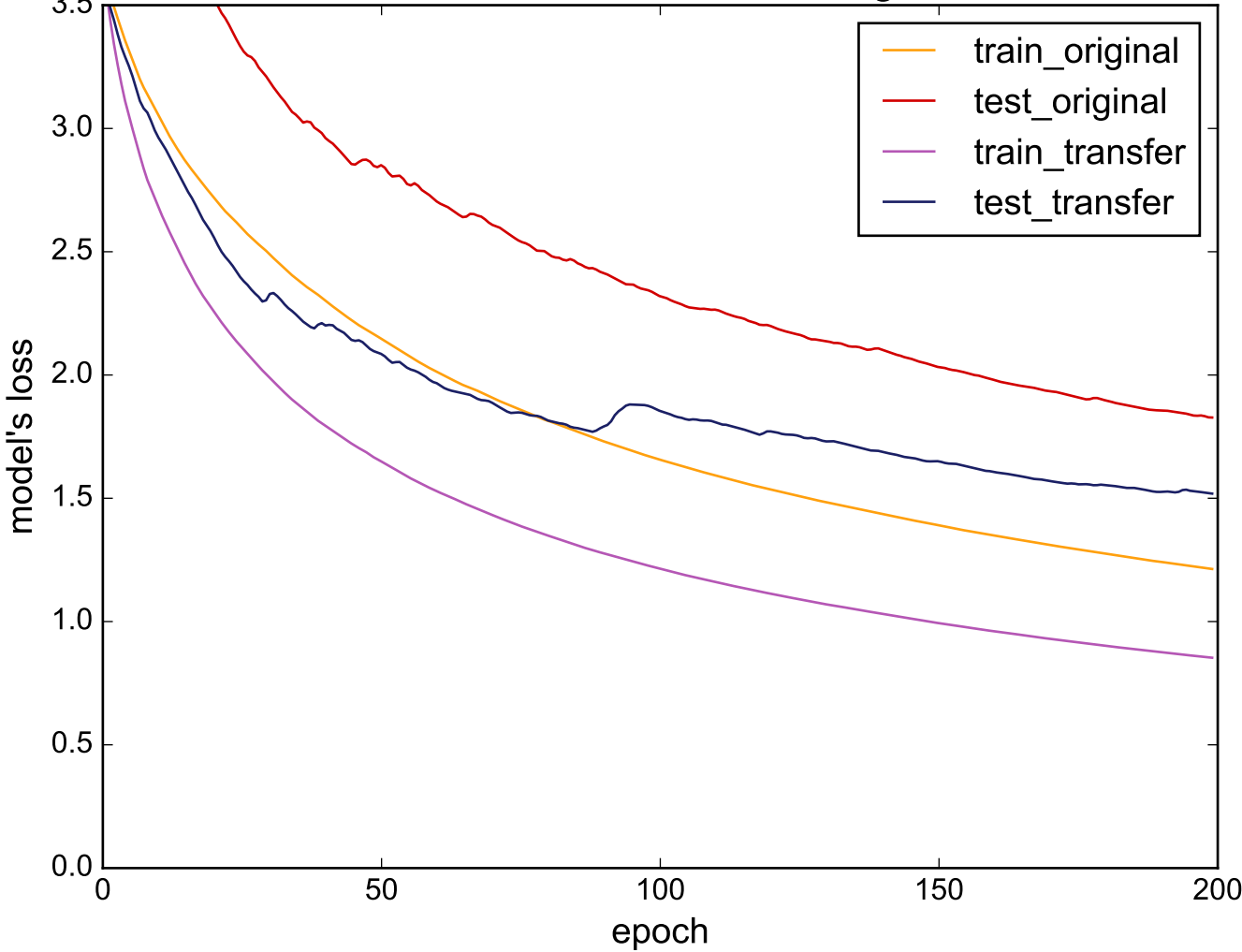
Source: MiddlePhalanxTW - Target: Adiac
