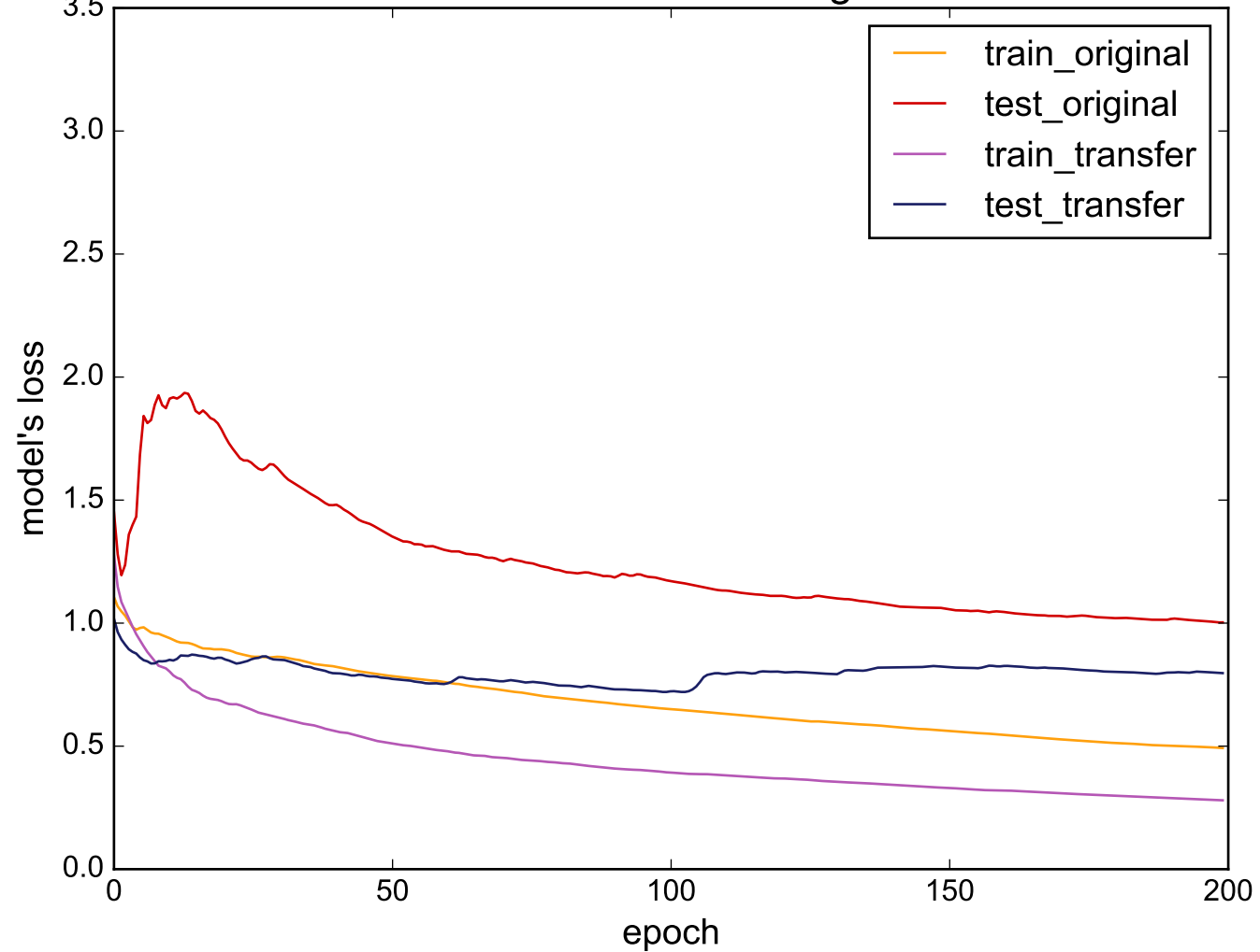
Source: MiddlePhalanxTW - Target: ArrowHead
