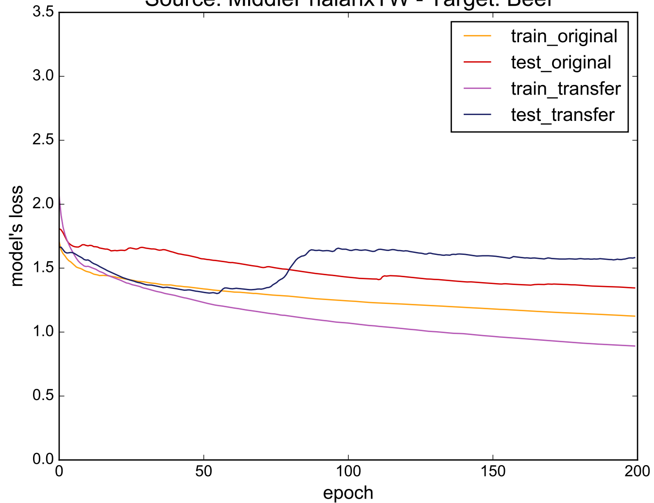
Source: MiddlePhalanxTW - Target: Beef
