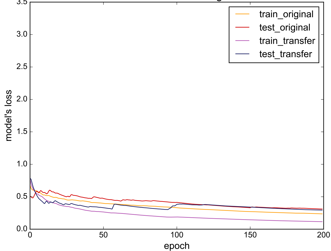
Source: MiddlePhalanxTW - Target: BirdChicken
