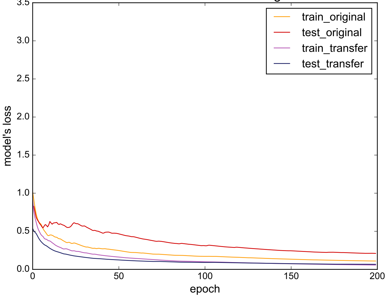
Source: MiddlePhalanxTW - Target: CBF
