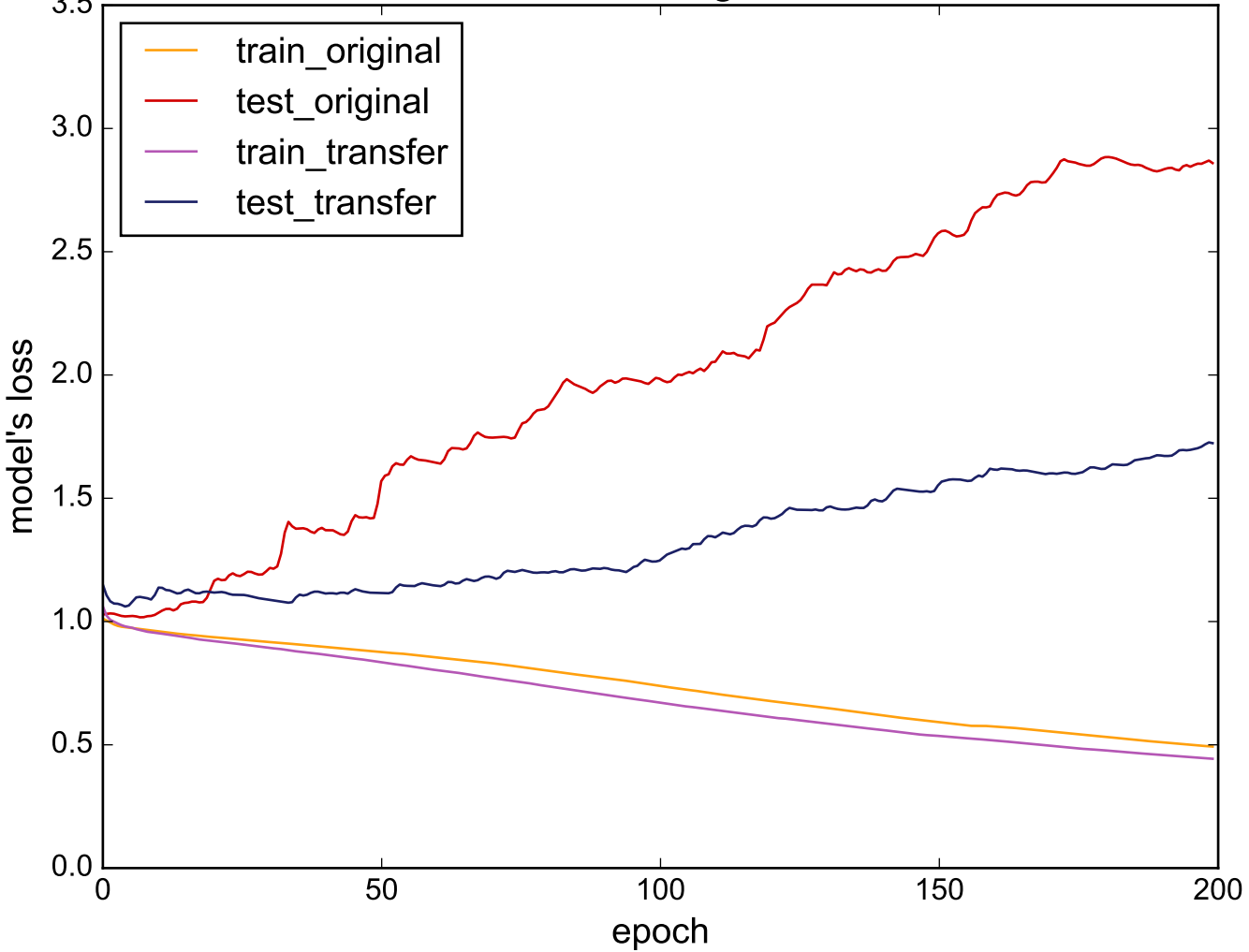
Source: MiddlePhalanxTW - Target: ChlorineConcentration
